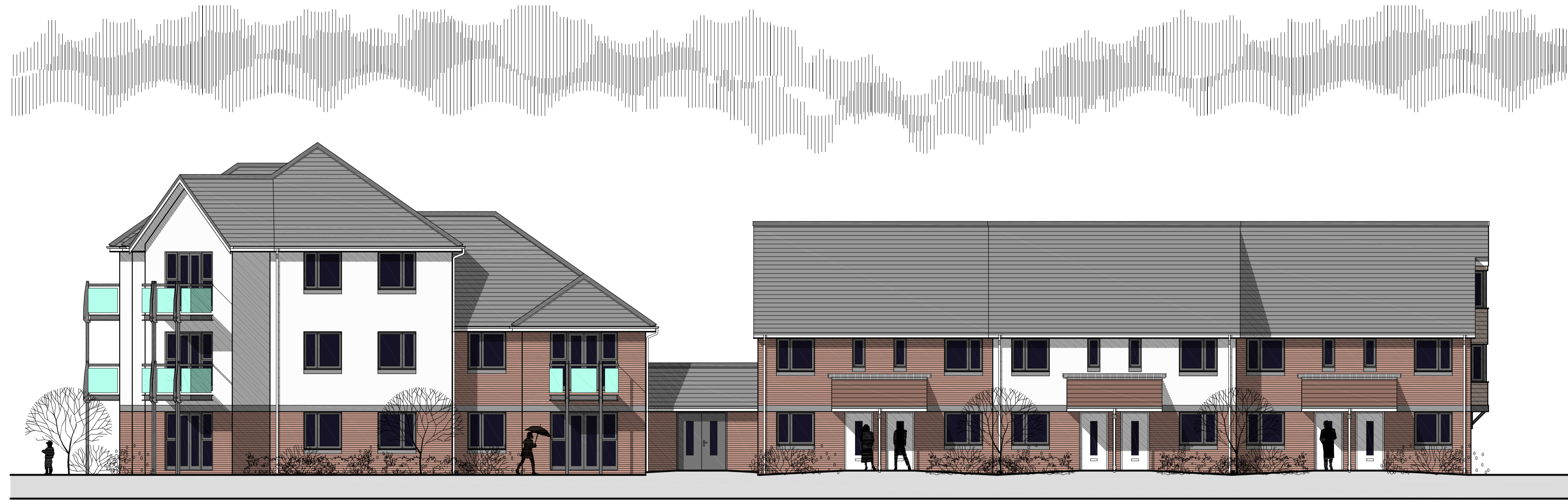
WEST ELEVATION 1:100 SCALE
